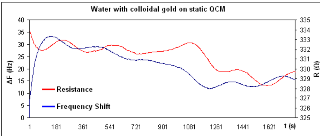
Fig.2. Static QCM date for water with Au colloidal
