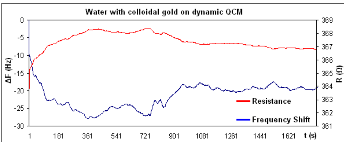
Fig.3. Dynamic QCM date for water with Au colloidal
