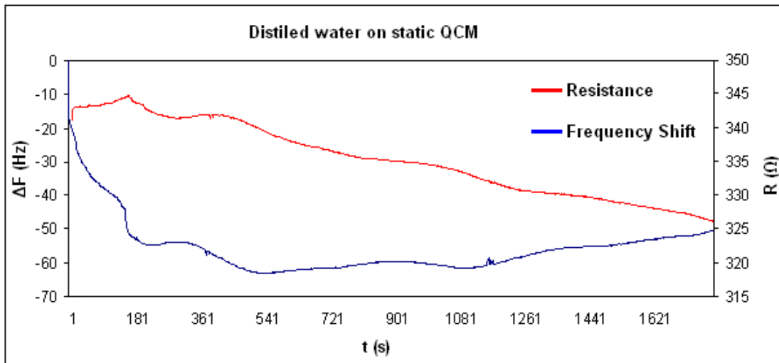
Fig.1. QCM date for pure water (distilled water)
