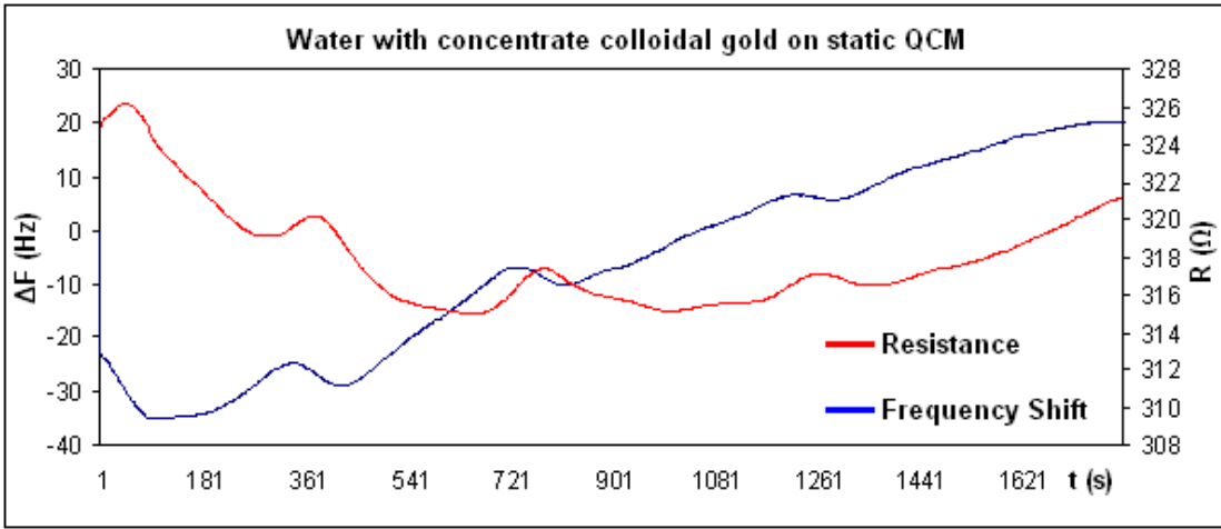
Fig.4. Static QCM data for water with Au colloidal
